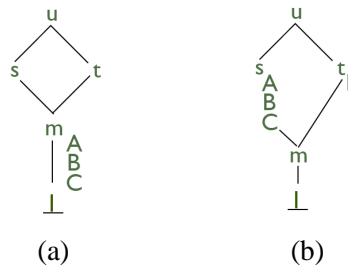
Figure 4: An illustration of (a) high mesh vs. (b) low mesh.
