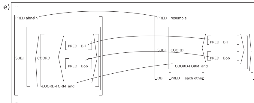
Figure 3: Alignment of Local F-structures
