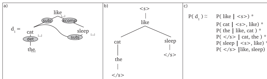
Figure 5: Dependency-Based Language Model Example for F-structure of The cat likes to sleep
